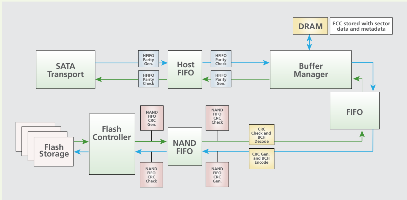
Figure 6: Client-specific data path protection
