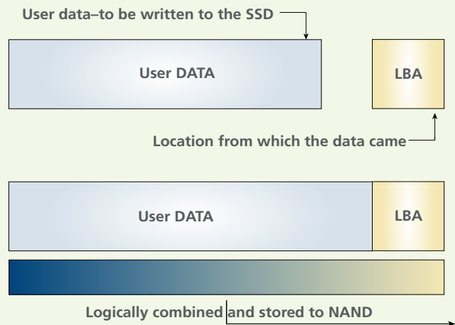
Figure 5: Writing data to the SSD
