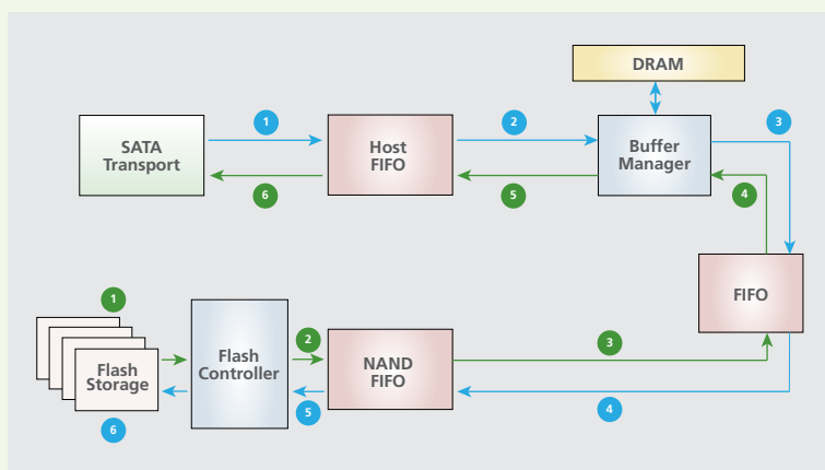
Figure 1: Typical data path for a SATA SSD
