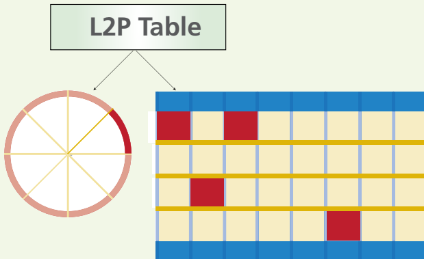
Figure 4: L2P table
