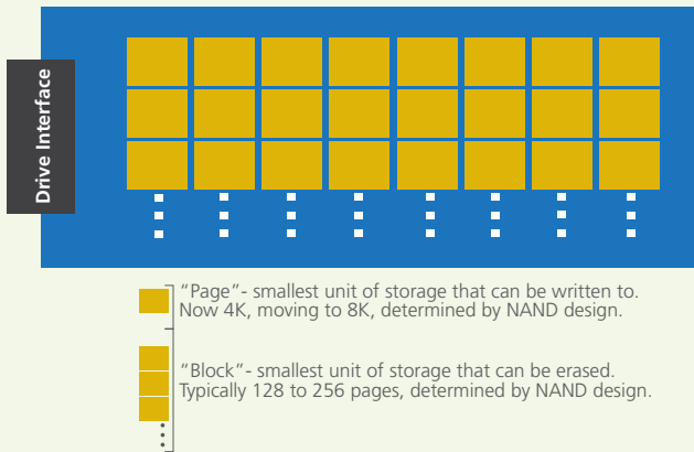
Figure 2: Simplified SSD diagram
