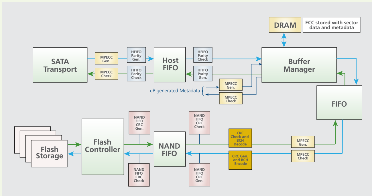
Figure 7: Enterprise-specific data path protection
